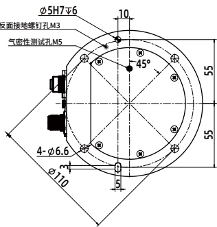
FR3C Pedestal diagram
