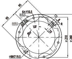
FR20 Pedestal diagram
