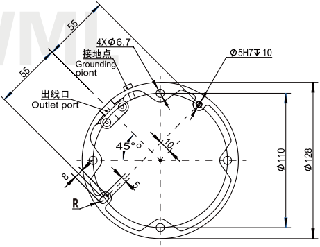
FR3WML Pedestal diagram
